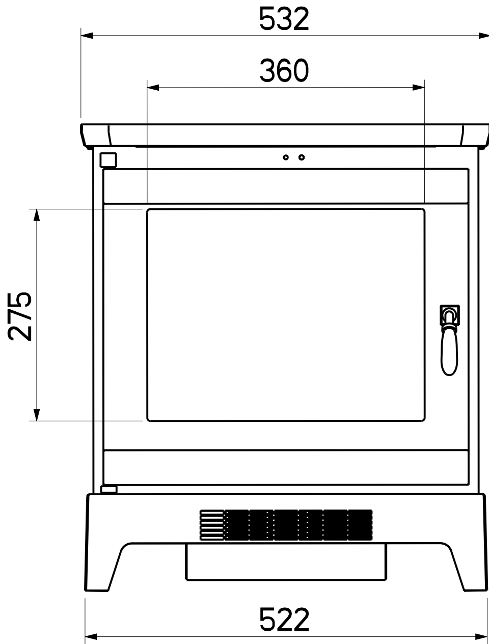
E-VR ROCHESTER STOVE ALL DIMENSIONS IN mm
