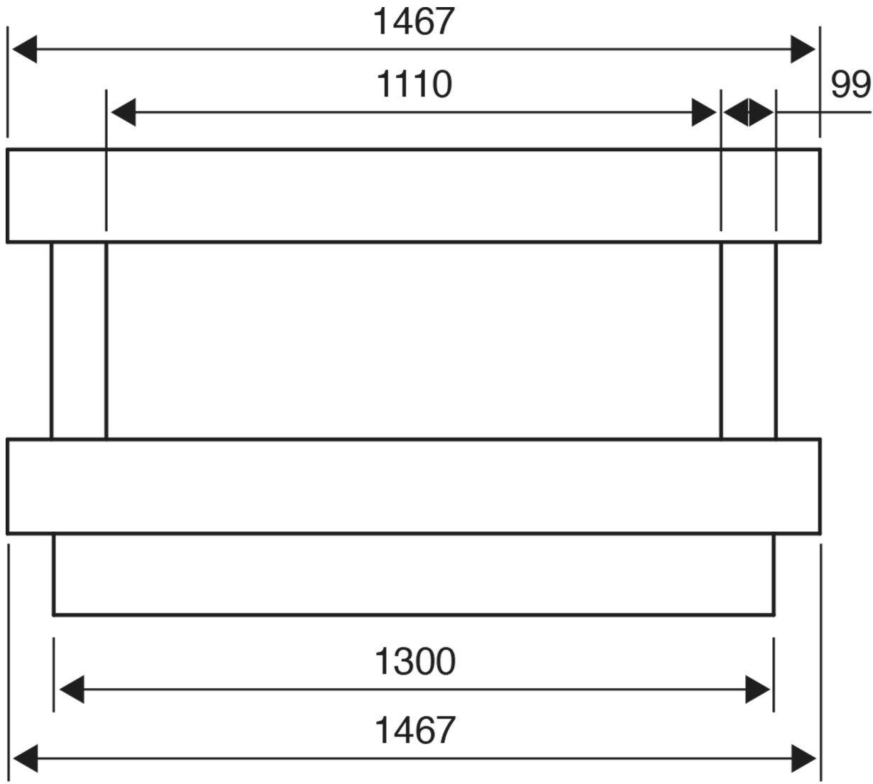
E-VR 1100 CARINO SUITE ALL DIMENSIONS IN mm
