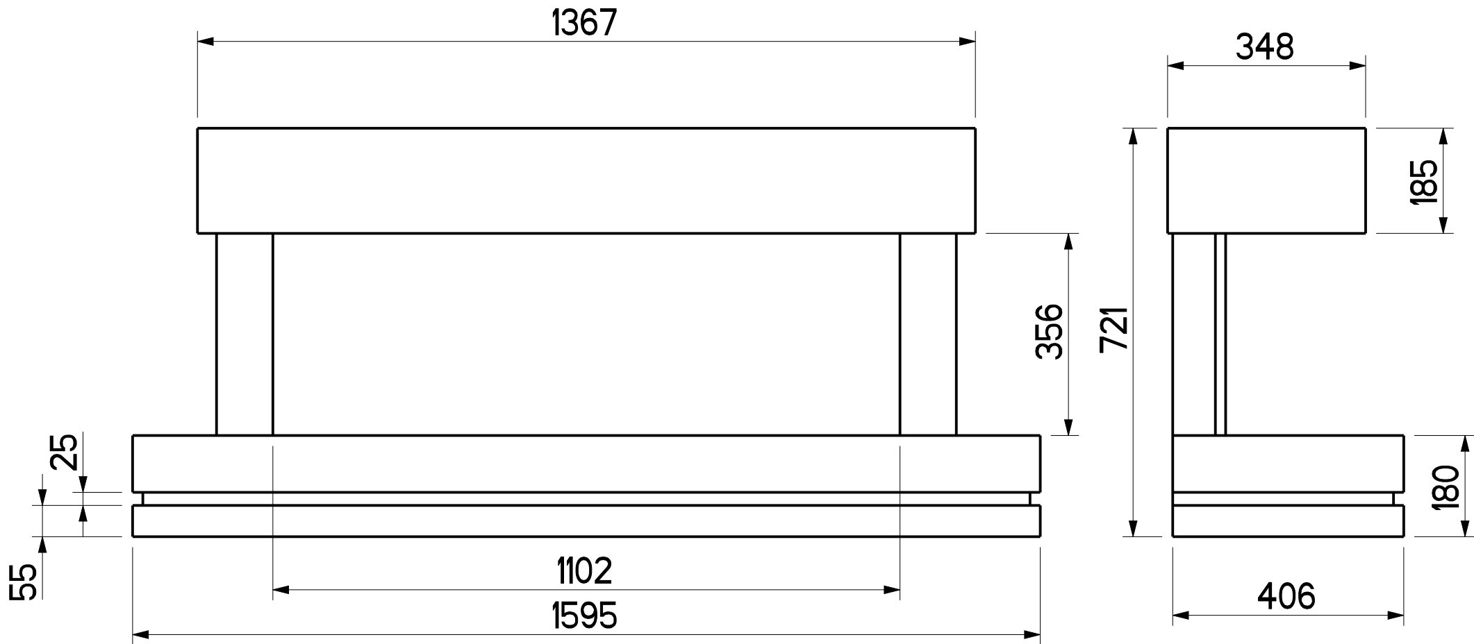
E-VR VOLARE 1100 SUITE ALL DIMENSIONS IN mm
