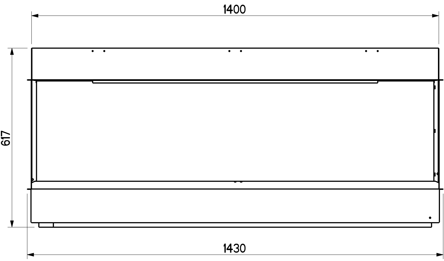
E-VR 1400 ALL DIMENSIONS IN mm
