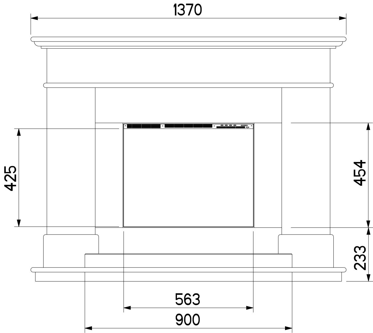
BOTICELLI ALL DIMENSIONS IN mm
